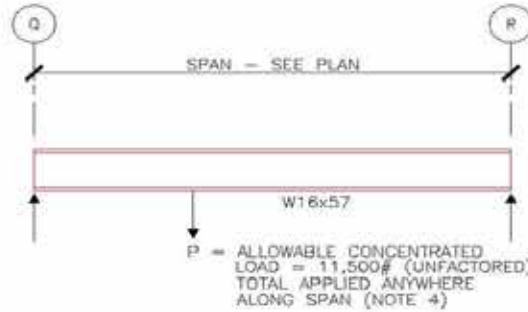
STAGE CENTER PURLIN
