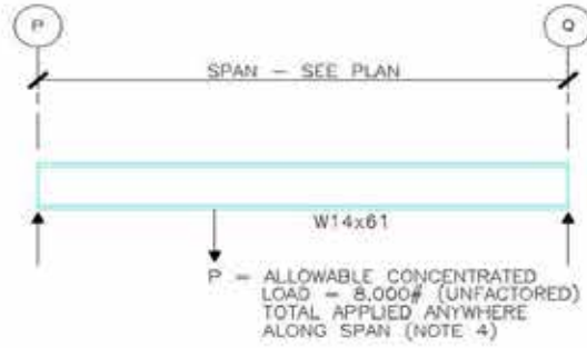
THEATRE AREA PURLIN
