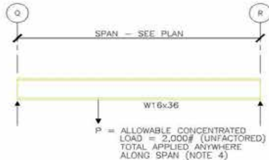
STAGE LEFT & RIGHT PURLIN
