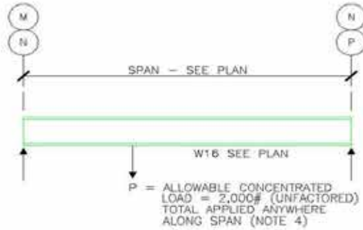
THEATRE AREA PURLIN
